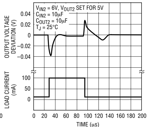
Output 2 Transient Response C_{BYP} = 0.01µF
