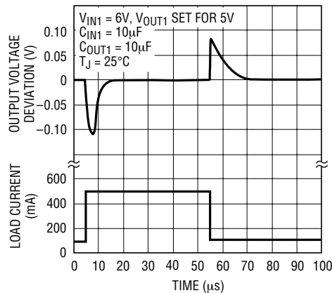
Output 1 Transient Response C_{BYP} = 0.01µF
