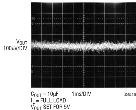
10Hz to 100kHz Output Noise C_{BYP} = 0.01µF
